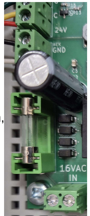
Fig 3, Fuse
