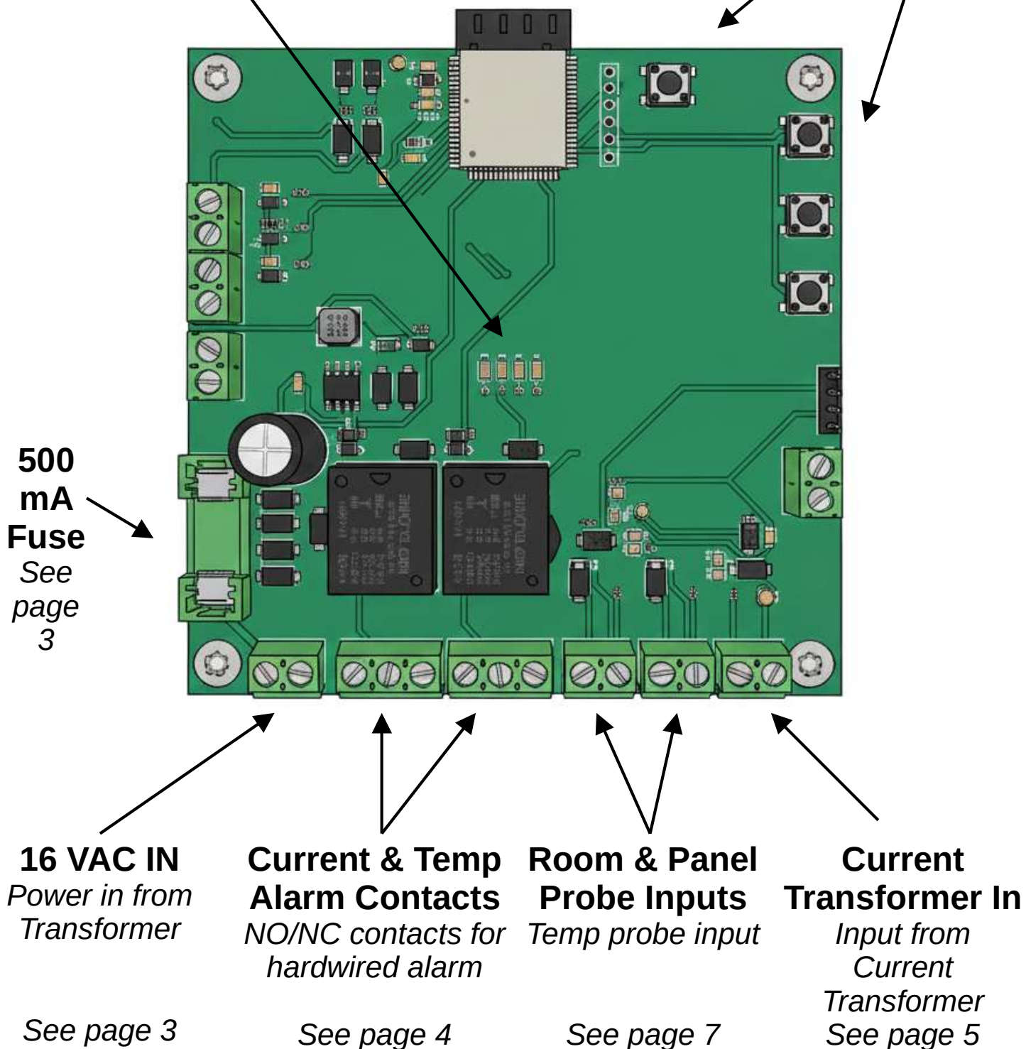
Fig 1, Board layout
